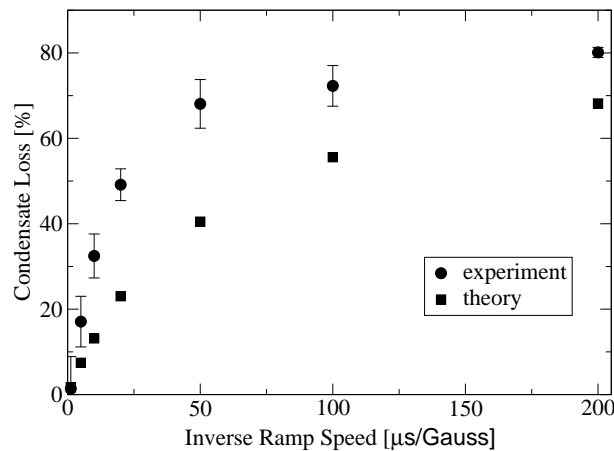
FIG. 1: Loss of atoms from a ^{85}\text{Rb} condensate at the end of a linear magnetic field ramp across the 155 Gauss Feshbach resonance as a function of the inverse ramp speed. The circles with error bars are the experimental data from Ref. [25]. The squares are determined from Eq. (9) using a cylindrical trap potential with the experimental trap frequencies.
